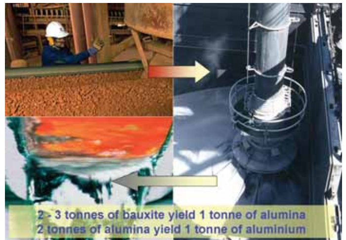
Figure 4: Processing of bauxite, production of alumina and aluminium
